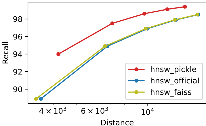
Recall vs Distance deep_10M_M32_ef100_k100
