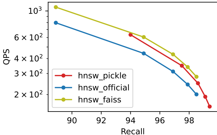
Recall vs QPS deep_10M_M32_ef100_k100
