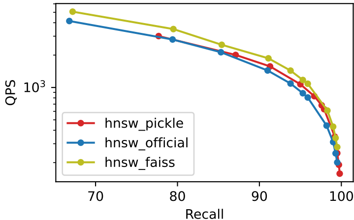
Recall vs QPS deep_10M_M32_ef100_k10
