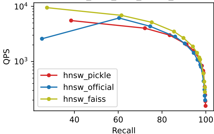
Recall vs QPS deep_10M_M32_ef100_k1
