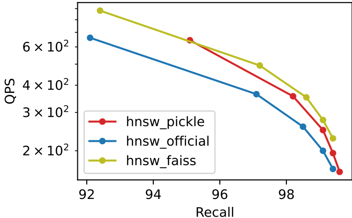
Recall vs QPS deep_10M_M32_ef300_k100
