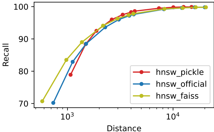
Recall vs Distance deep_10M_M32_ef300_k10
