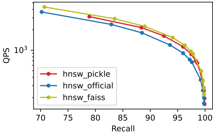
Recall vs QPS deep_10M_M32_ef300_k10
