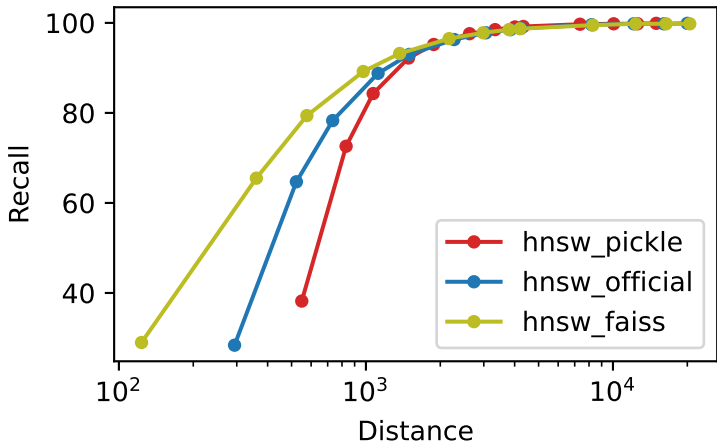
Recall vs Distance deep_10M_M32_ef300_k1
