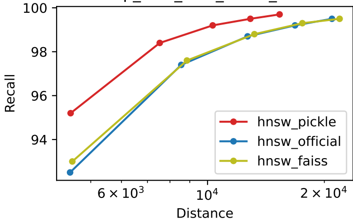
Recall vs Distance deep_10M_M32_ef500_k100
