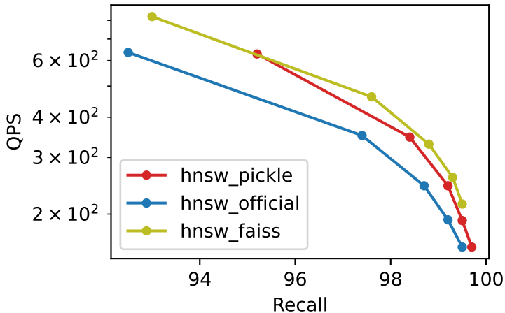
Recall vs QPS deep_10M_M32_ef500_k100
