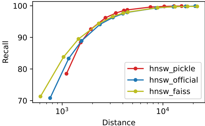
Recall vs Distance deep_10M_M32_ef500_k10
