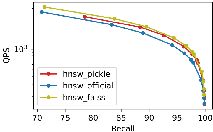
Recall vs QPS deep_10M_M32_ef500_k10
