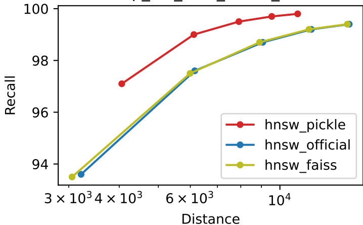
Recall vs Distance deep_1M_M32_ef100_k100
