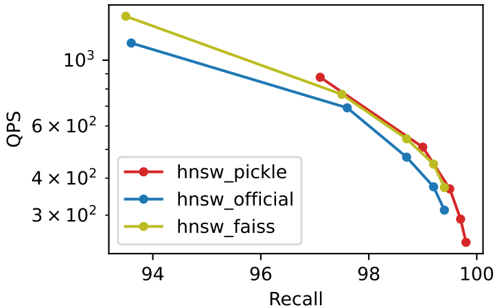
Recall vs QPS deep_1M_M32_ef100_k100
