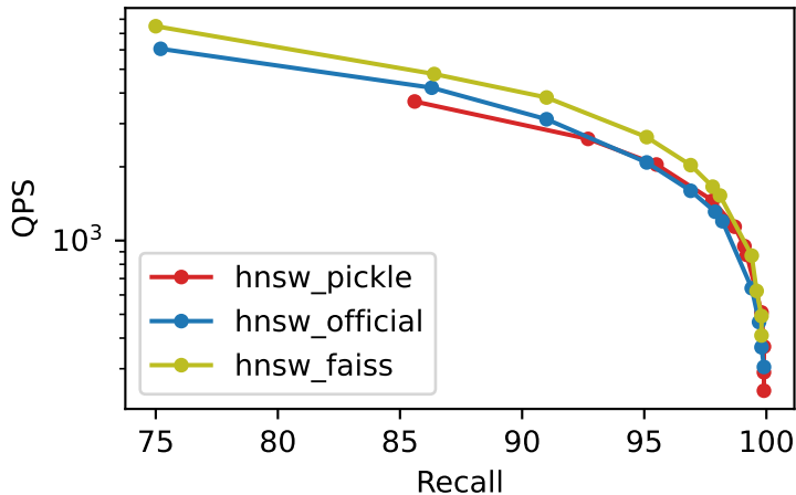
Recall vs QPS deep_1M_M32_ef100_k10
