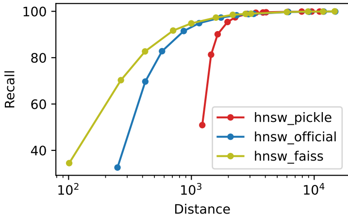
Recall vs Distance deep_1M_M32_ef100_k1
