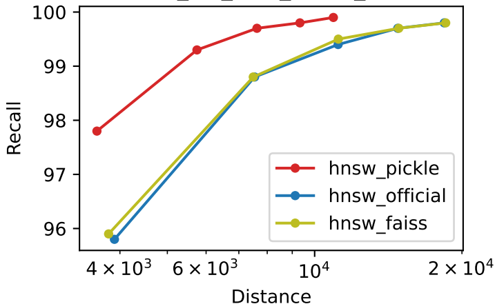
Recall vs Distance deep_1M_M32_ef300_k100
