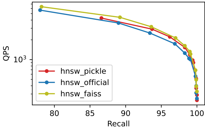
Recall vs QPS deep_1M_M32_ef300_k10
