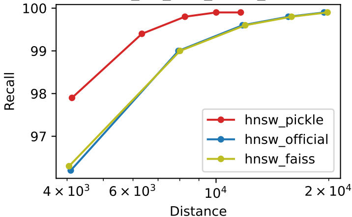
Recall vs Distance deep_1M_M32_ef500_k100
