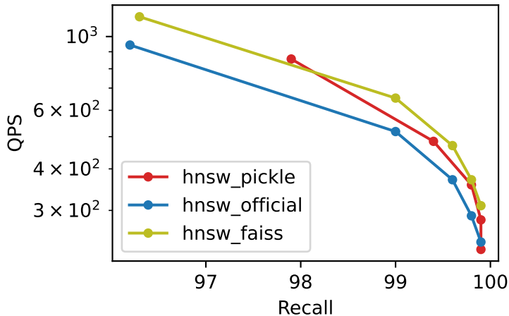
Recall vs QPS deep_1M_M32_ef500_k100
