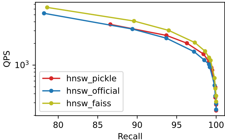
Recall vs QPS deep_1M_M32_ef500_k10
