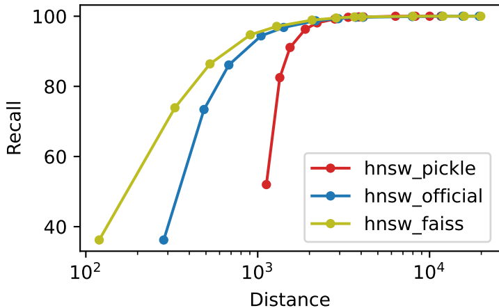
Recall vs Distance deep_1M_M32_ef500_k1
