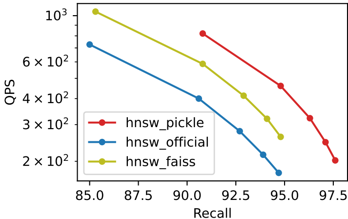
Recall vs QPS msspacev_10M_M32_ef100_k100
