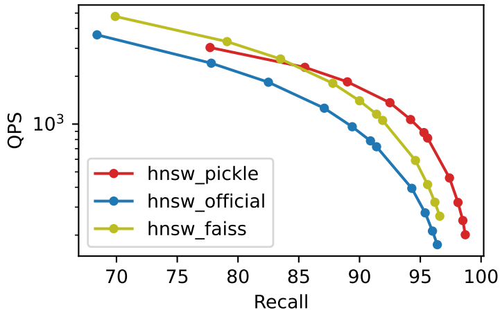
Recall vs QPS msspacev_10M_M32_ef100_k10
