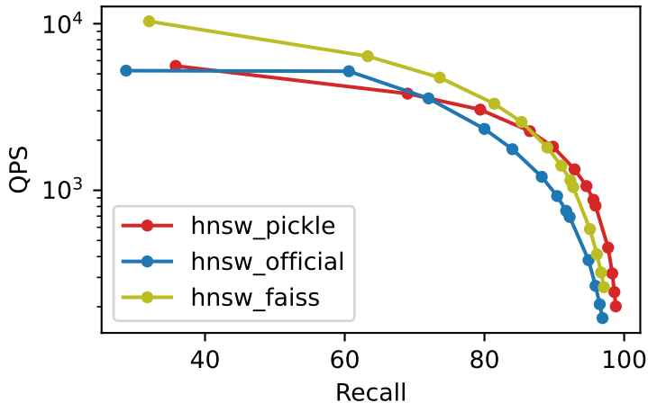
Recall vs QPS msspacev_10M_M32_ef100_k1
