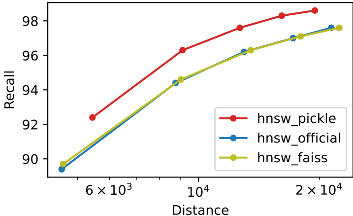
Recall vs Distance msspacev_10M_M32_ef300_k100
