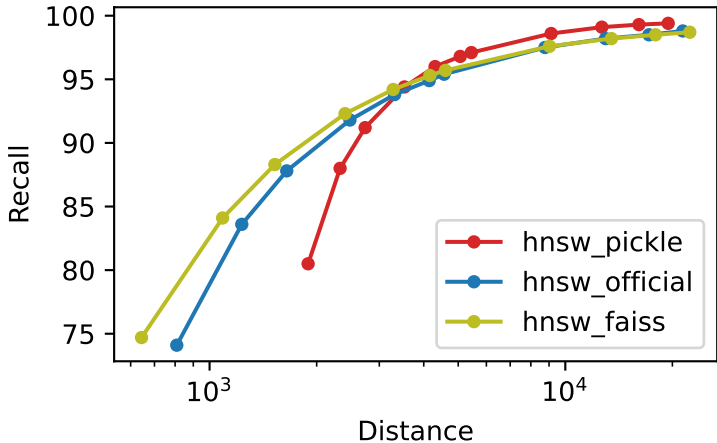
Recall vs Distance msspacev_10M_M32_ef300_k10
