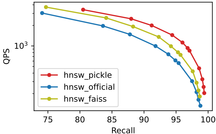
Recall vs QPS msspacev_10M_M32_ef300_k10
