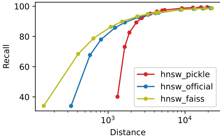
Recall vs Distance msspacev_10M_M32_ef300_k1
