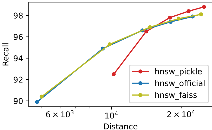
Recall vs Distance msspacev_10M_M32_ef500_k100
