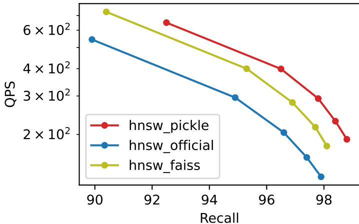
Recall vs QPS msspacev_10M_M32_ef500_k100
