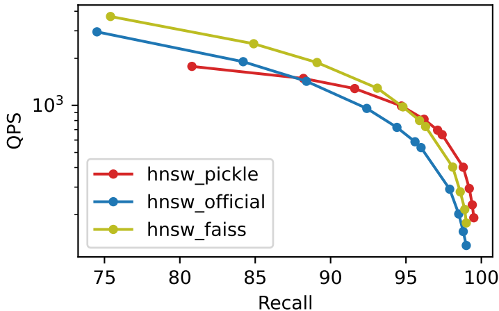
Recall vs QPS msspacev_10M_M32_ef500_k10
