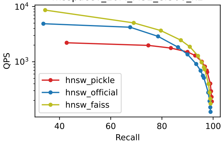
Recall vs QPS msspacev_10M_M32_ef500_k1
