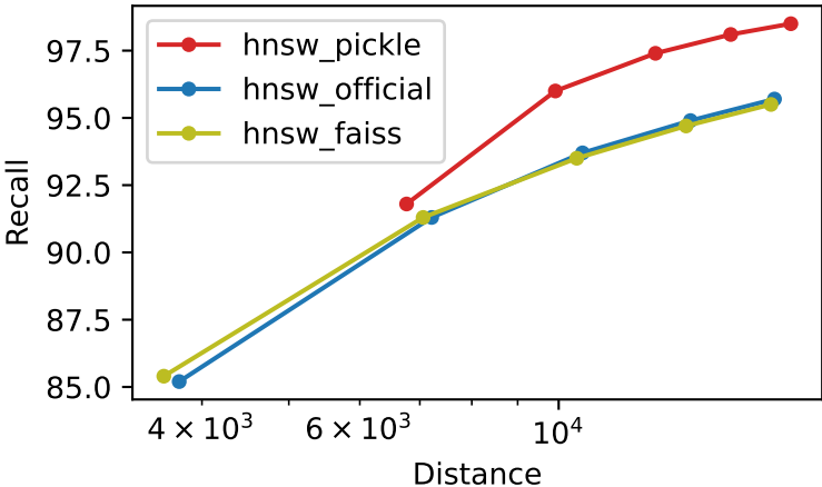
Recall vs Distance msspacev_1M_M32_ef100_k100
