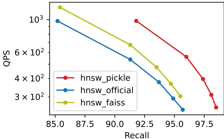
Recall vs QPS msspacev_1M_M32_ef100_k100
