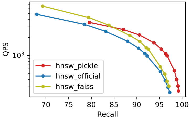
Recall vs QPS msspacev_1M_M32_ef100_k10
