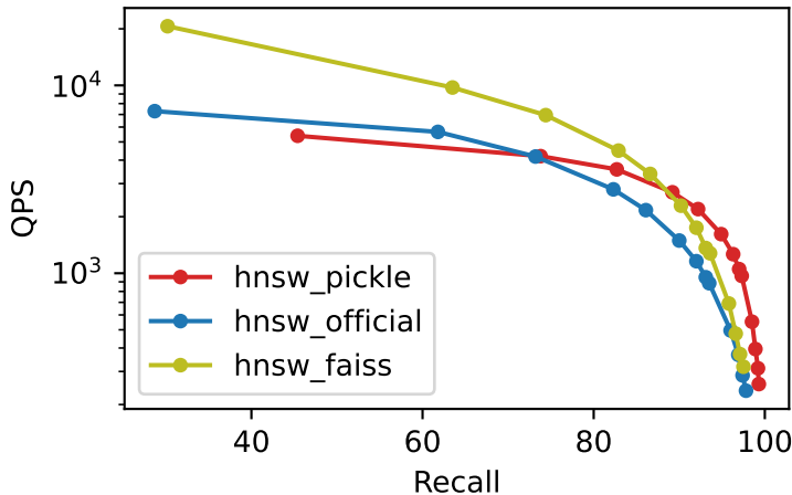
Recall vs QPS msspacev_1M_M32_ef100_k1
