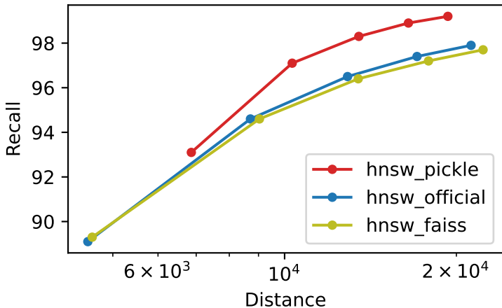
Recall vs Distance msspacev_1M_M32_ef300_k100
