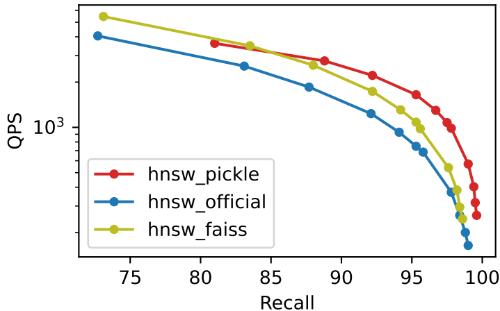
Recall vs QPS msspacev_1M_M32_ef300_k10
