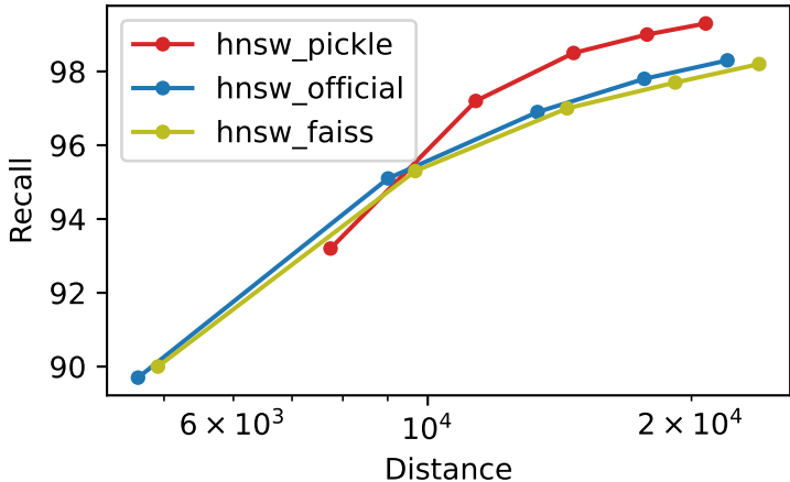
Recall vs Distance msspacev_1M_M32_ef500_k100
