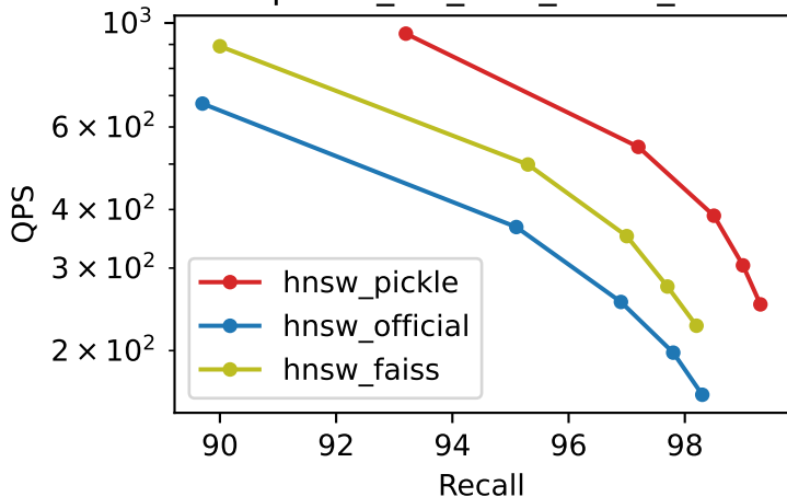
Recall vs QPS msspacev_1M_M32_ef500_k100
