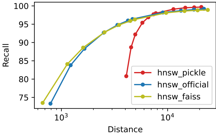
Recall vs Distance msspacev_1M_M32_ef500_k10
