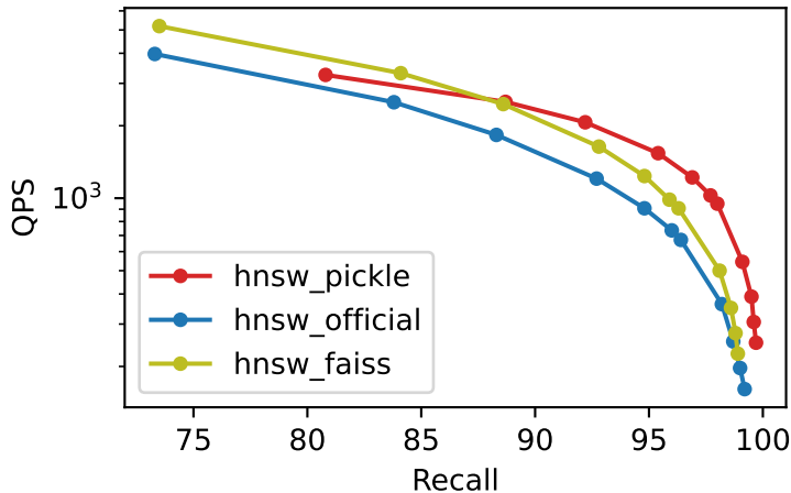
Recall vs QPS msspacev_1M_M32_ef500_k10
