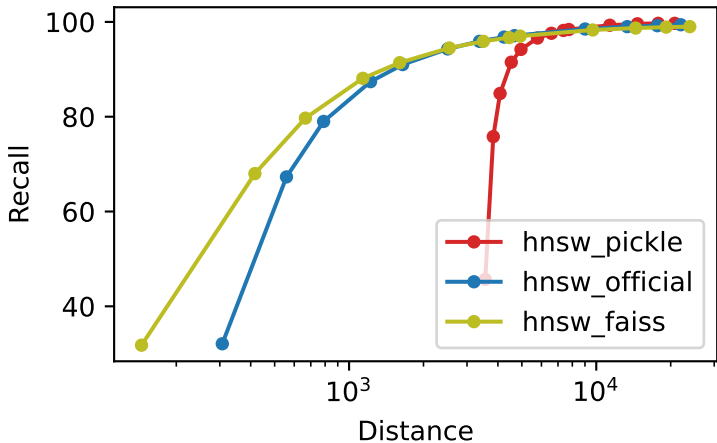
Recall vs Distance msspacev_1M_M32_ef500_k1
