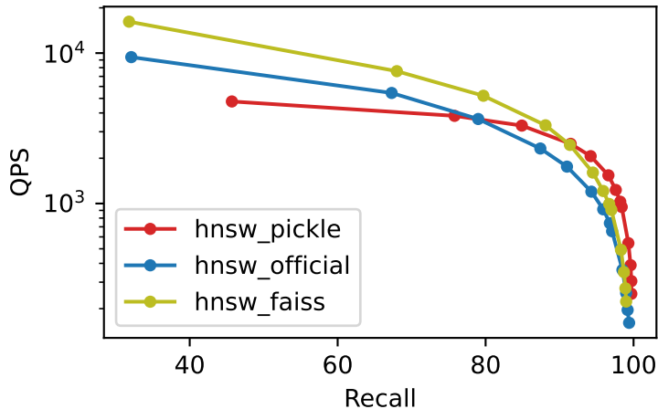
Recall vs QPS msspacev_1M_M32_ef500_k1
