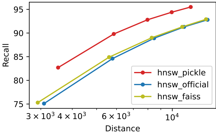
Recall vs Distance text2image_10M_M32_ef100_k100
