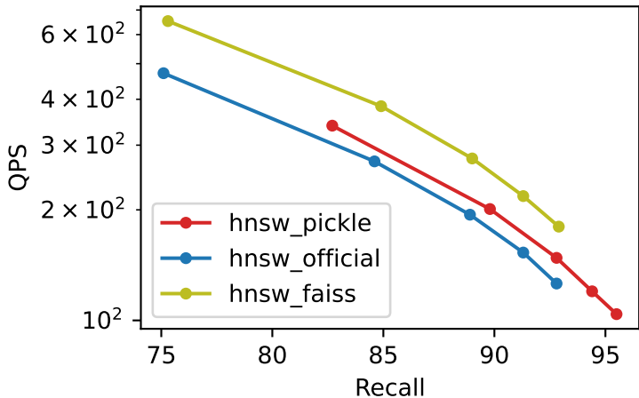
Recall vs QPS text2image_10M_M32_ef100_k100
