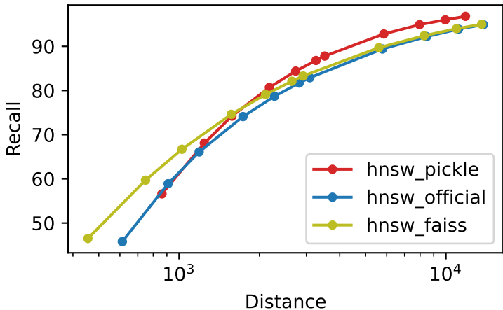
Recall vs Distance text2image_10M_M32_ef100_k10
