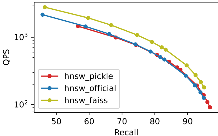
Recall vs QPS text2image_10M_M32_ef100_k10
