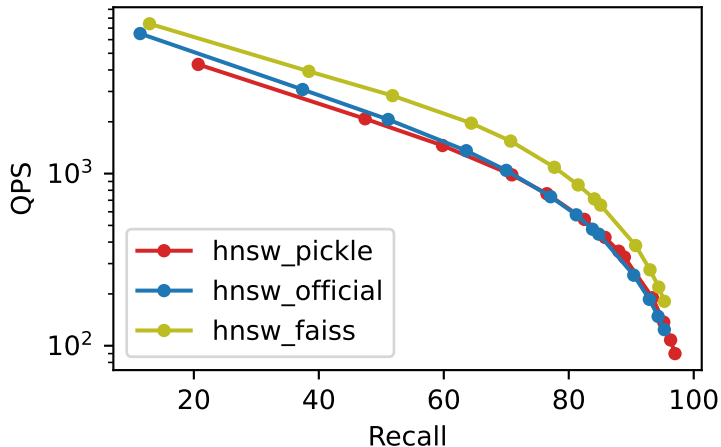
Recall vs QPS text2image_10M_M32_ef100_k1
